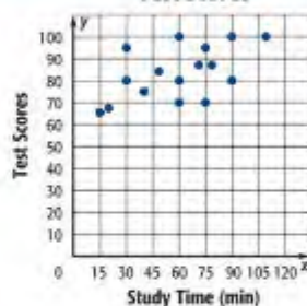
Test Scores
