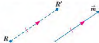
Point R' is a translation of point R along translation vector m .
