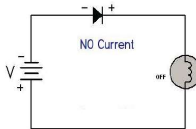
(B) diode placed in reverse bias
