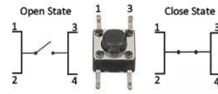
(B) Pushbutton Switch symbol (OFF)
