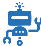
Teachable Machine
